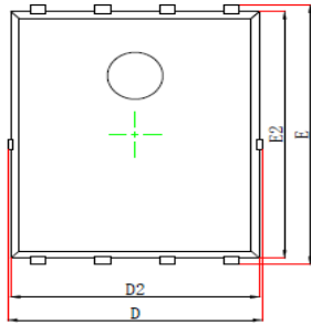
Top View [顶视图]
